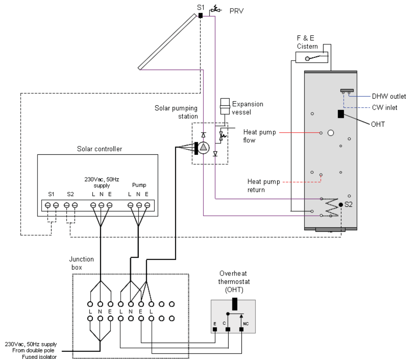
Typical schematic wiring diagram and system configuration for the Torrent GreenHeat HP-solar.
